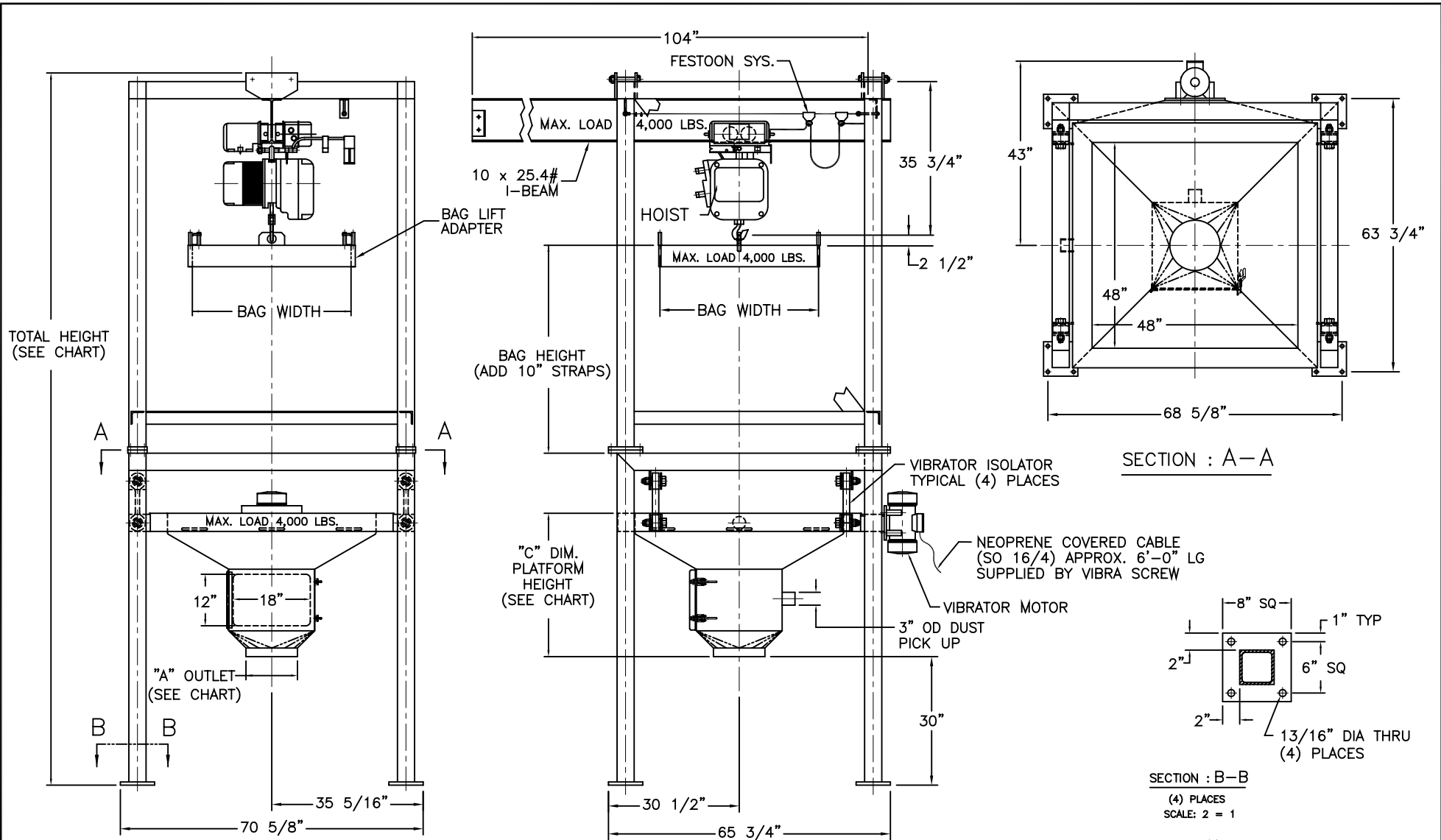
TOTAL HEIGHT WITH BAG LENGTH SHOWN (INCLUDES 10" STRAPS)
