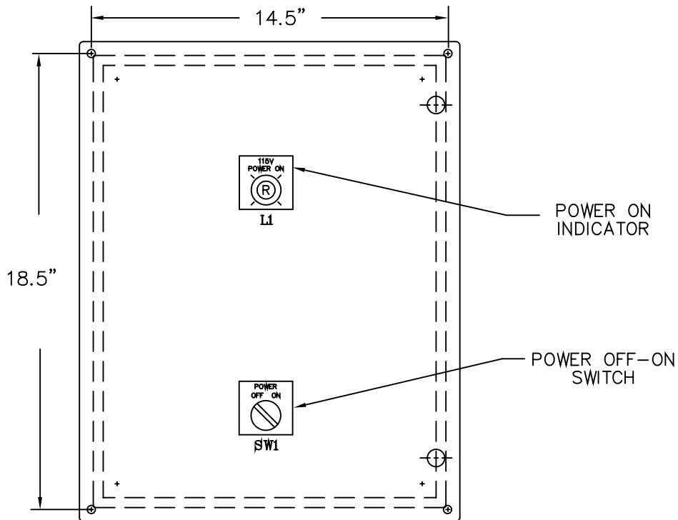
WALL MOUNT ENCLOSURE DIM.: 20" H x 16" W x 6" D'P.
