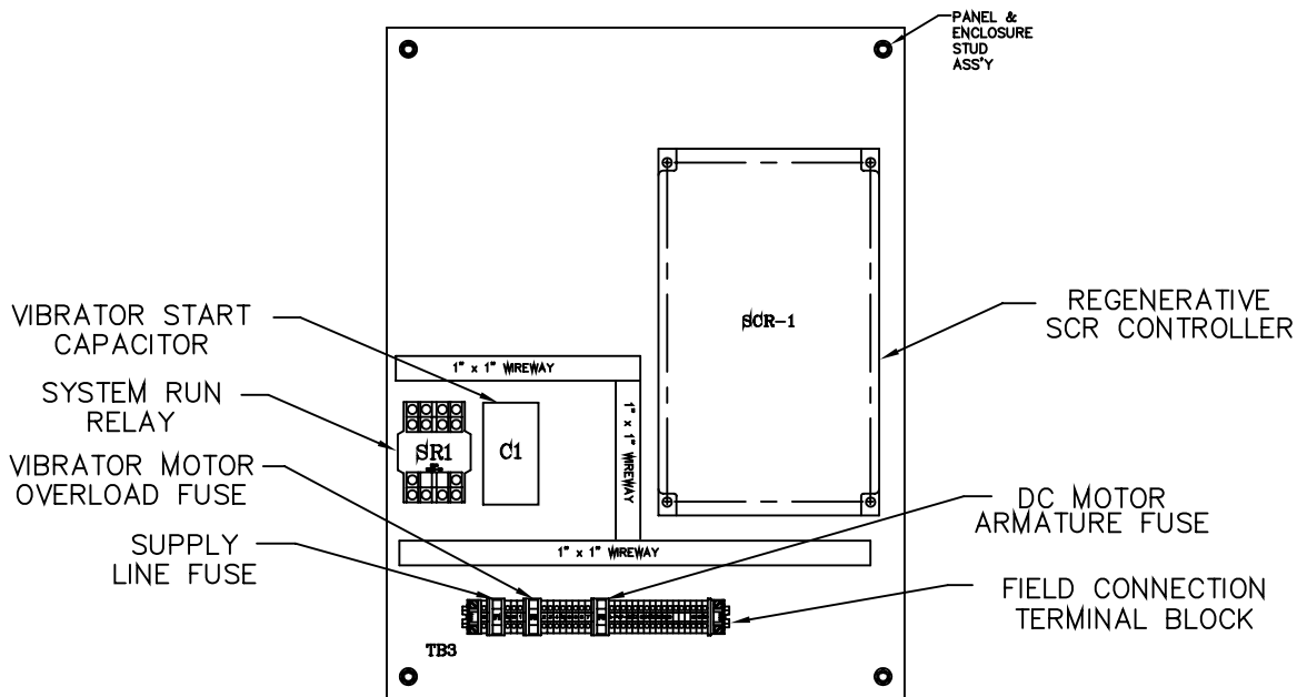
PANEL LAYOUT
