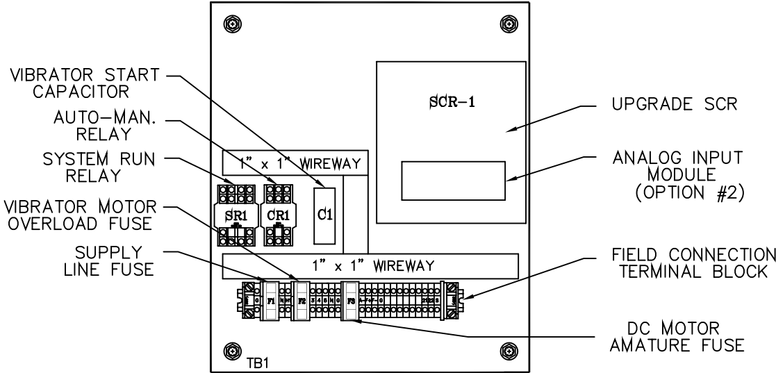
WALL MOUNT ENCLOSURE DIM.: 20" x 16" x 6"
