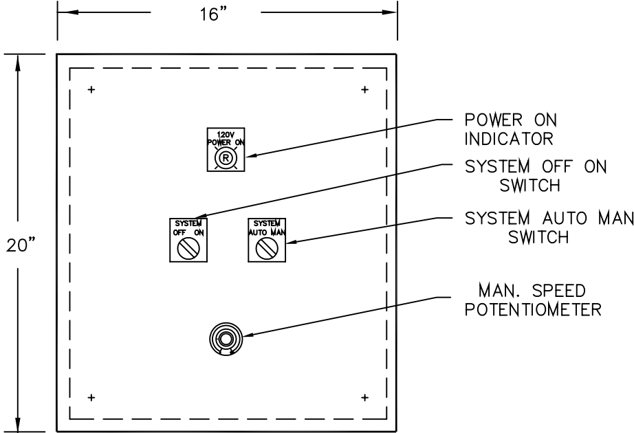
WALL MOUNT ENCLOSURE DIM.: 20" x 16" x 6"
