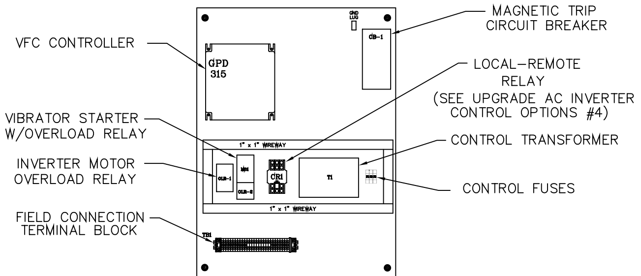
PANEL LAYOUT
