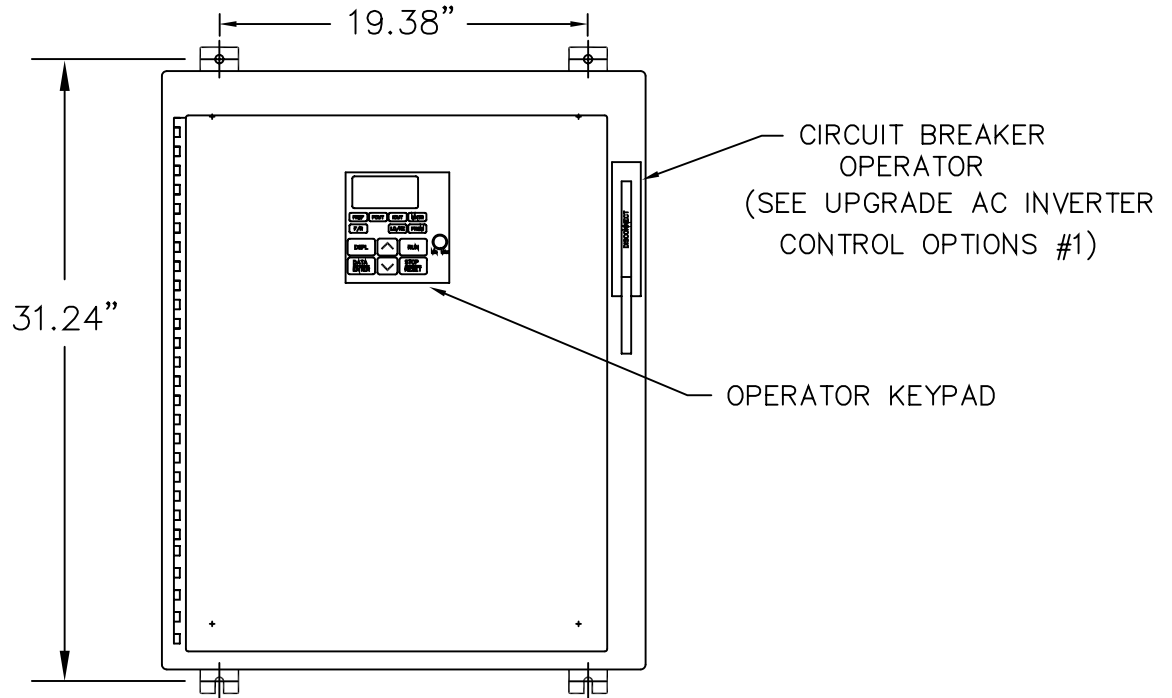
WALL MOUNT ENCLOSURE DIM.: 30" x 25.38" x 8" (AVAILABLE: NEMA 4/12 & 4X)
