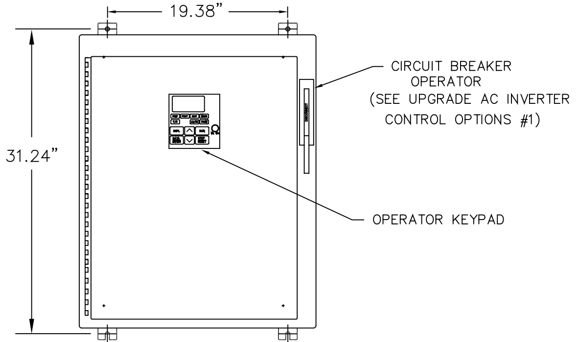
WALL MOUNT ENCLOSURE DIM.: 30" x 25.38" x 8" (AVAILABLE: NEMA 4/12 & 4X)
