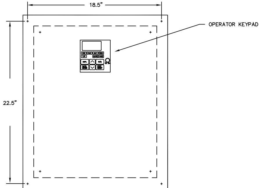
WALL MOUNT ENCLOSURE
