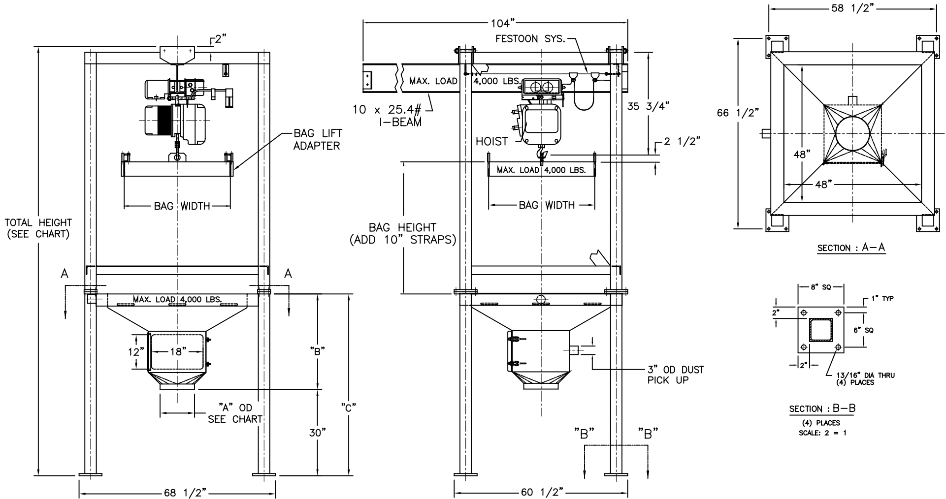
TOTAL HEIGHT WITH BAG LENGTH SHOWN (INCLUDES 10" STRAPS)
