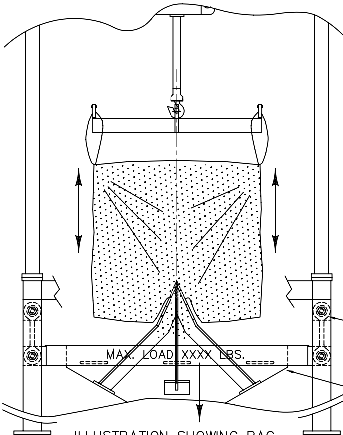
ILLUSTRATION SHOWING BAG BEING LOWERED AND PUNCTURED
