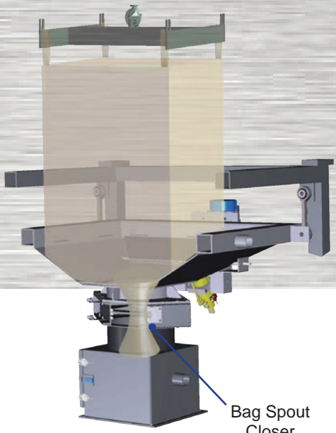
Bag Spout Closer Pinch Valve
